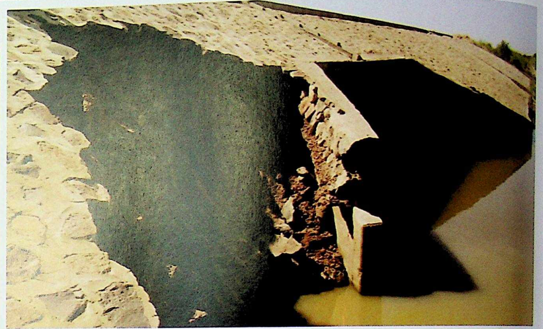
DAMAGES CAUSED BY THE FLOOD
