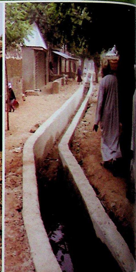
CONSTRUCTION OF DRAINAGES AND CULVERTS AT LIMAWA QUARTERS, DUTSE LOCAL GOVERNMENT AREA
