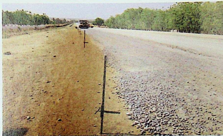
STONE BASE COURSE PAVING
