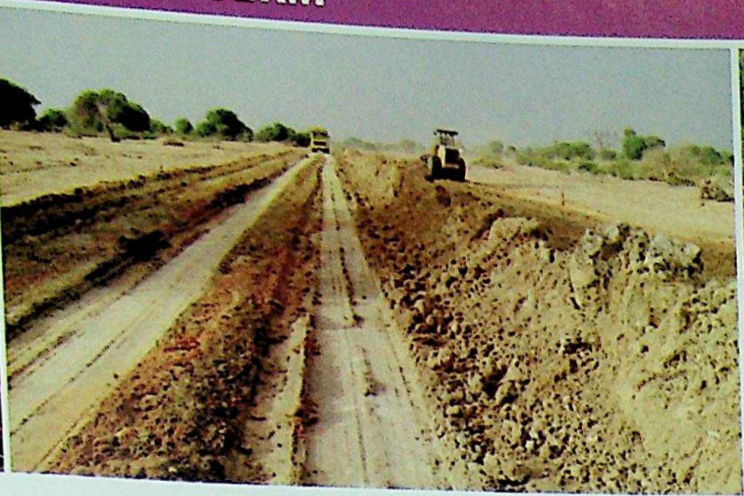
GRADING OF FILLING MATERIAL
