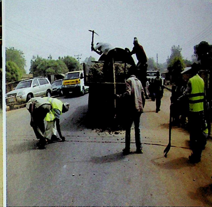
CONSTRUCTION OF SPEED BREAKERS IN COLLABORATION WITH FERMA AND FRSC AT APPROPRIATE LOCATION ON KANO – BIRNIN KUDU – KARI ROAD
