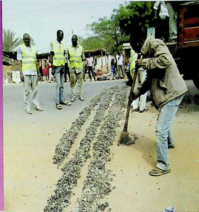
CONSTRUCTION OF SPEED BREAKERS IN COLLABORATION WITH FERMA AND FRSC AT APPROPRIATE LOCATION ON KANO – BIRNIN KUDU – KARI ROAD
