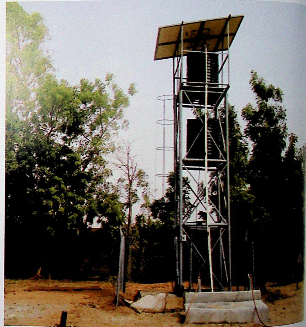
Solar borehole at Great Green Wall project site, Bajoda, Sule Tankarkar LGA
