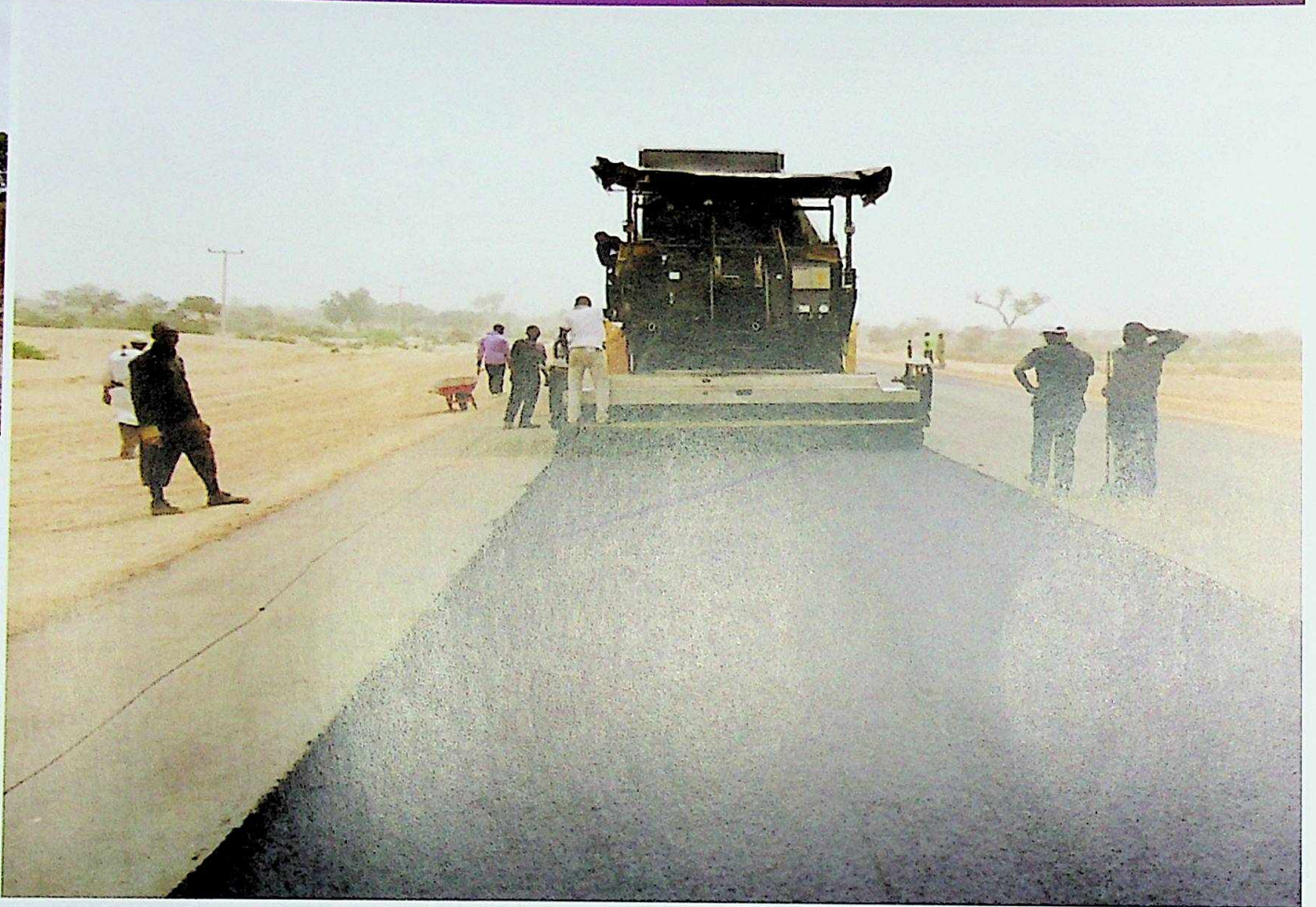
ASPHALTIC PAVING AND FINISHING
