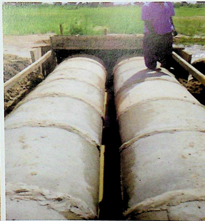
EXCAVATION AND CONSTRUCTION OF 2 CELL RING CULVERT
