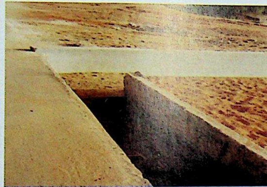
FAILED EMBANKMENT THREATENING THE PAVEMENT AT KADAITA
