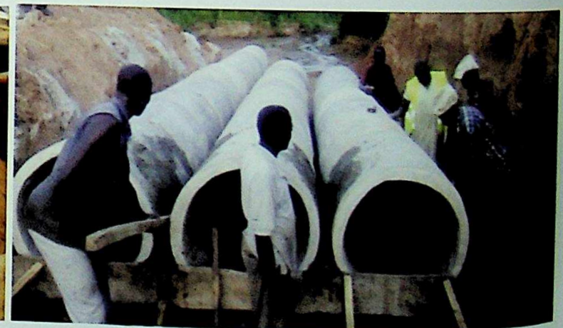
WORKS IN PROGRESS AT GADAMA CULVERT(NO.2)
