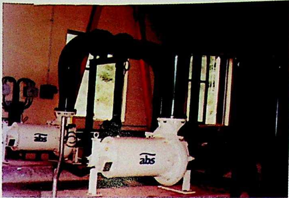
Eleyele Water Supply Scheme Low-Lift Pumps
